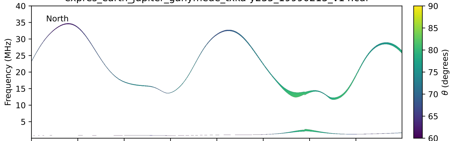
expres_earth_jupiter_ganymede_txka-y235_19990213_v14.cdf
