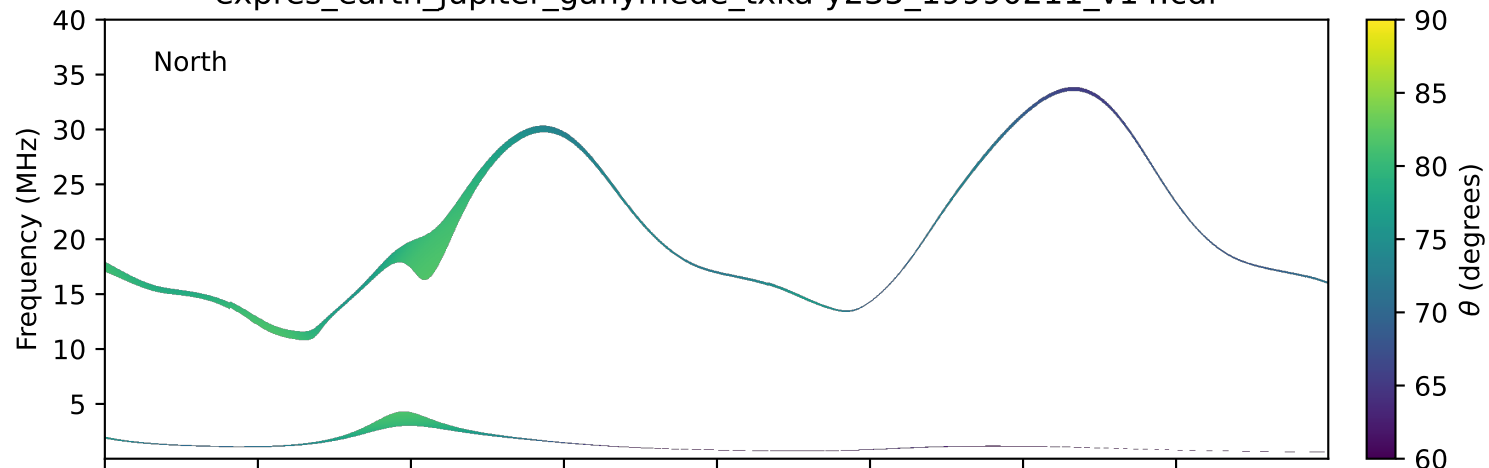
expres_earth_jupiter_ganymede_txka-y235_19990211_v14.cdf
