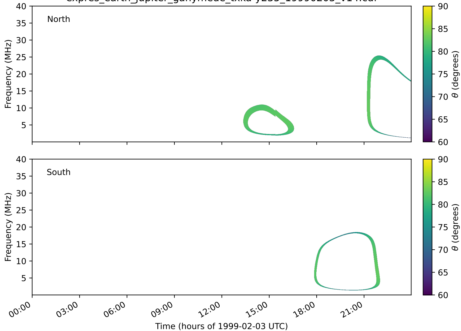
expres_earth_jupiter_ganymede_txka-y235_19990203_v14.cdf
