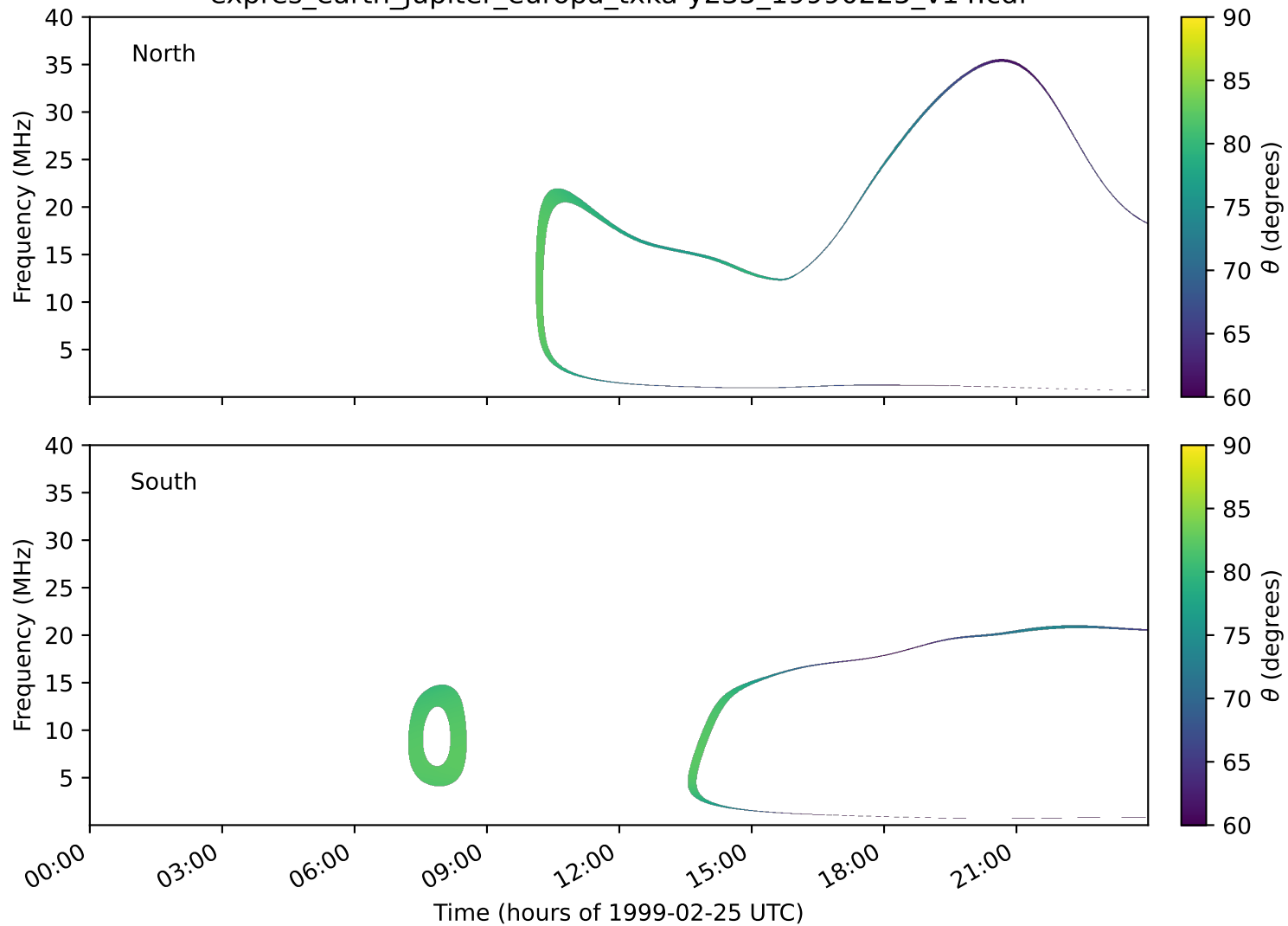
expres_earth_jupiter_europa_txka-y235_19990225_v14.cdf
