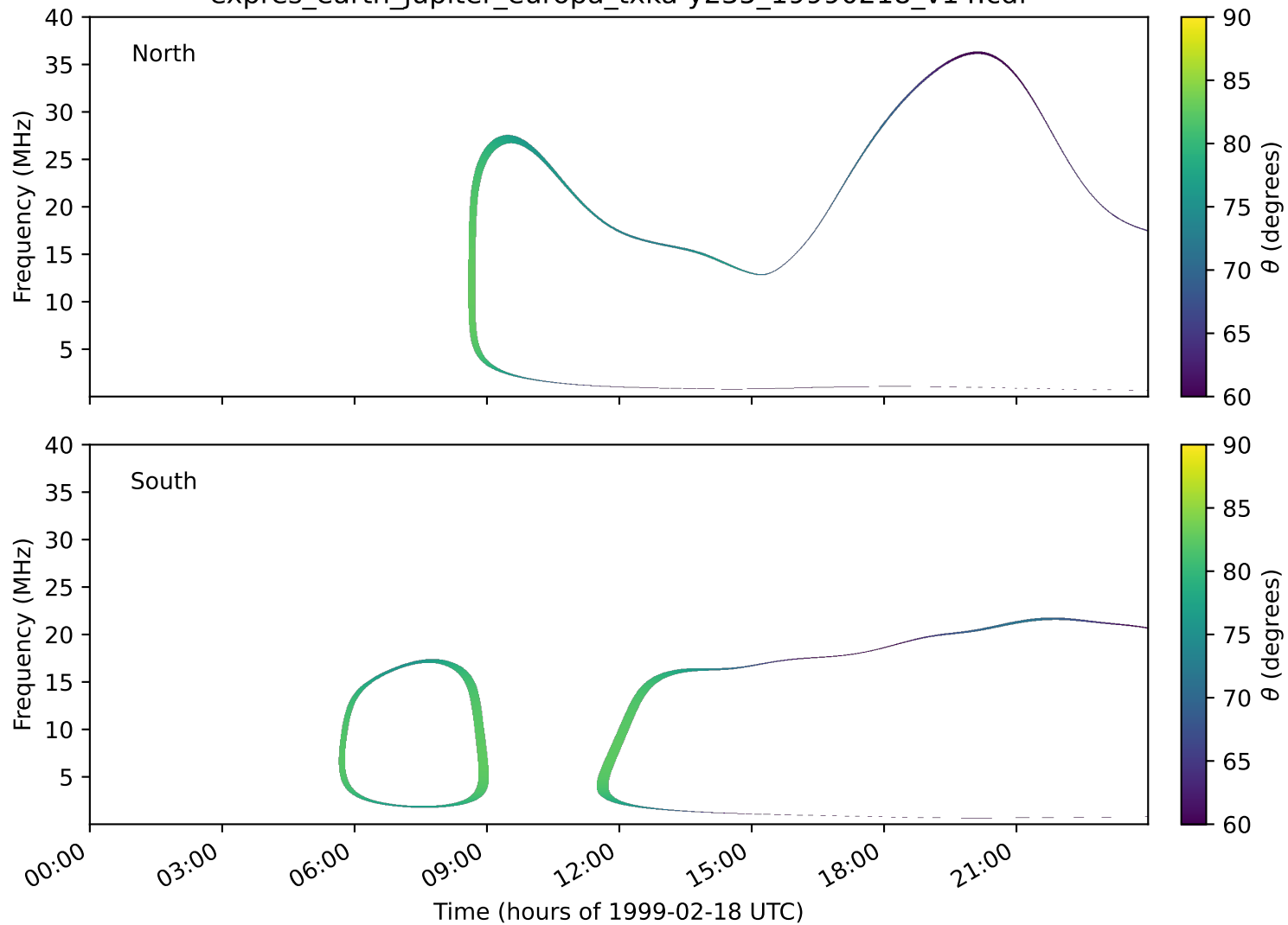
expres_earth_jupiter_europa_txka-y235_19990218_v14.cdf
