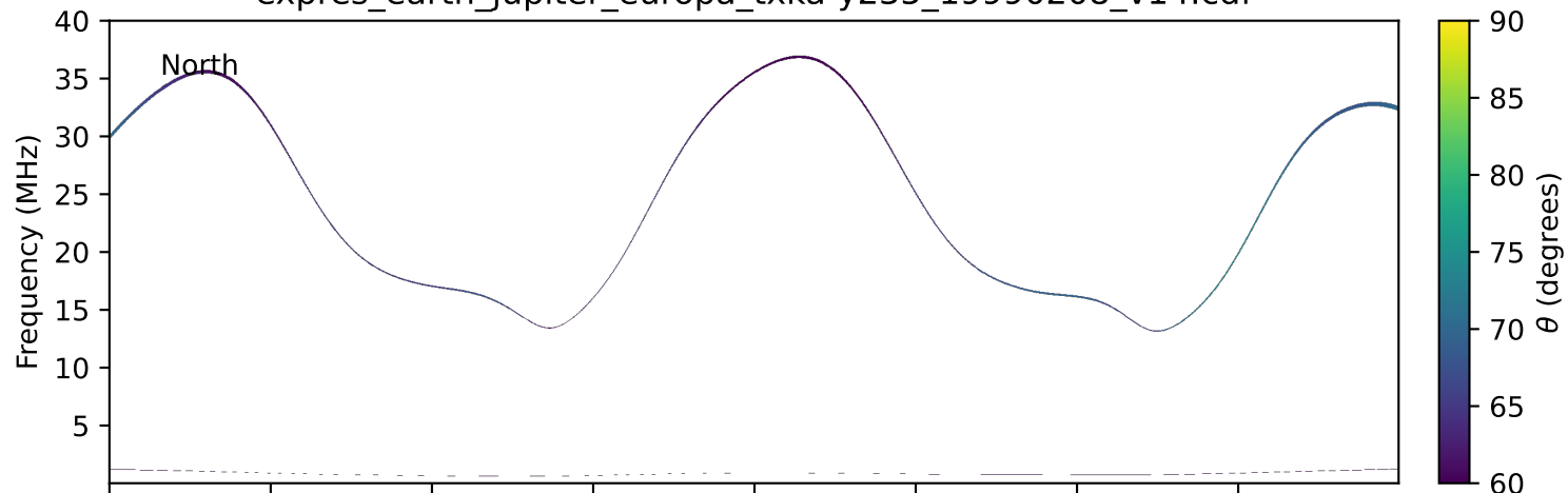
expres_earth_jupiter_europa_txka-y235_19990208_v14.cdf
