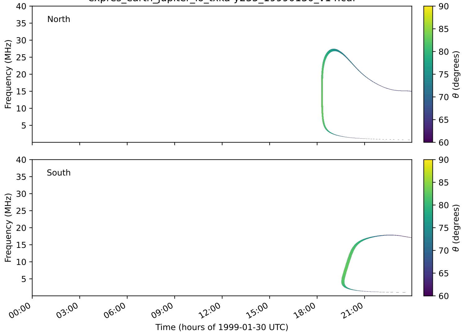
expres_earth_jupiter_io_txka-y235_19990130_v14.cdf
