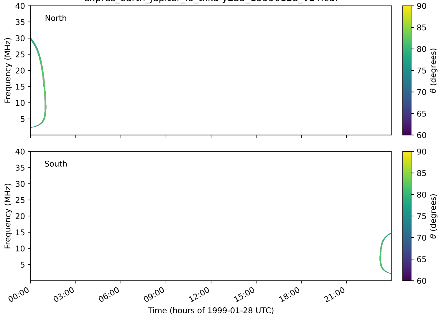
expres_earth_jupiter_io_txka-y235_19990128_v14.cdf
