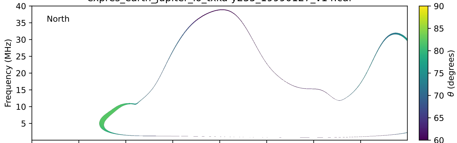
expres_earth_jupiter_io_txka-y235_19990127_v14.cdf
