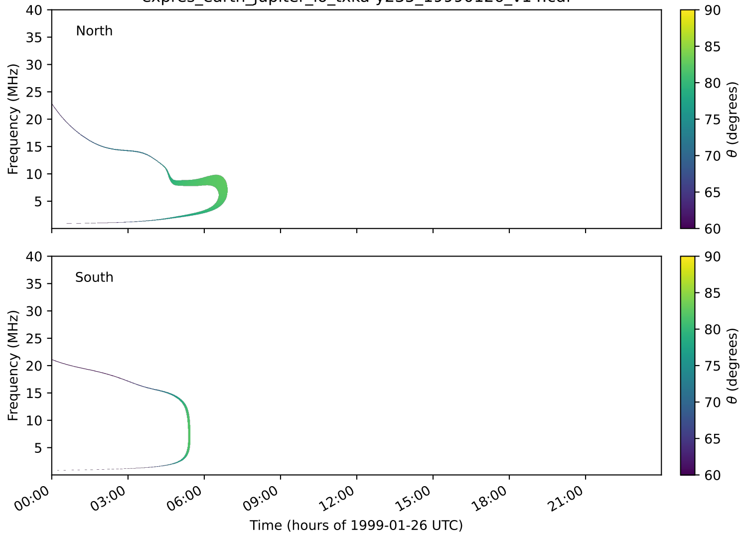
expres_earth_jupiter_io_txka-y235_19990126_v14.cdf
