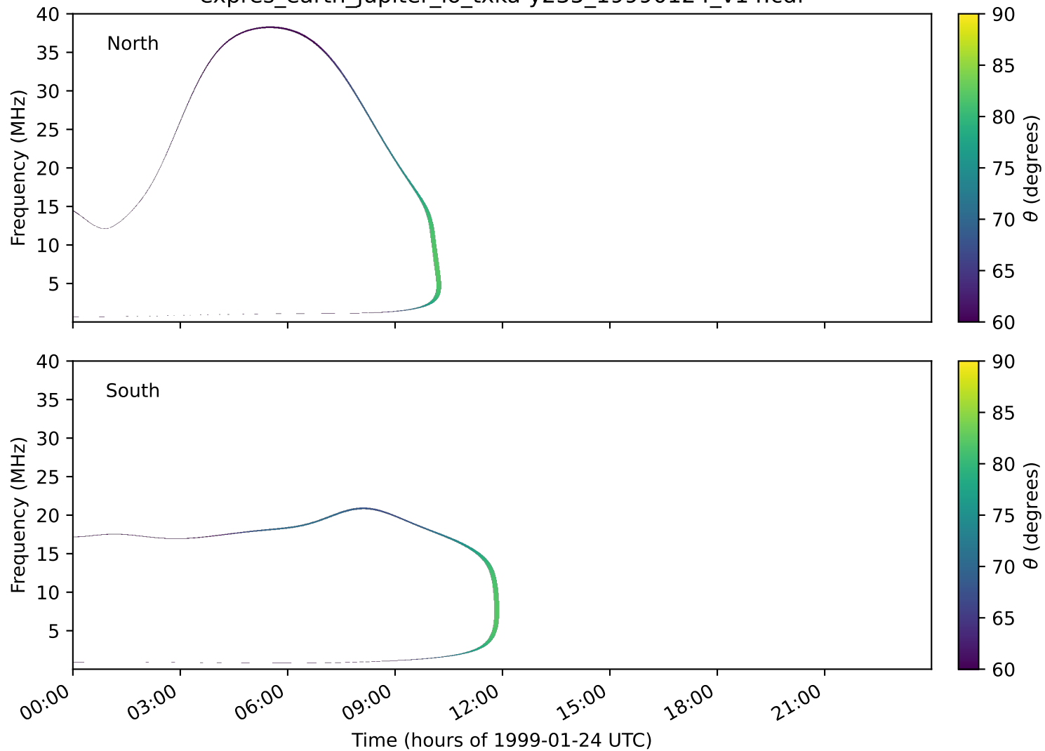
expres_earth_jupiter_io_txka-y235_19990124_v14.cdf
