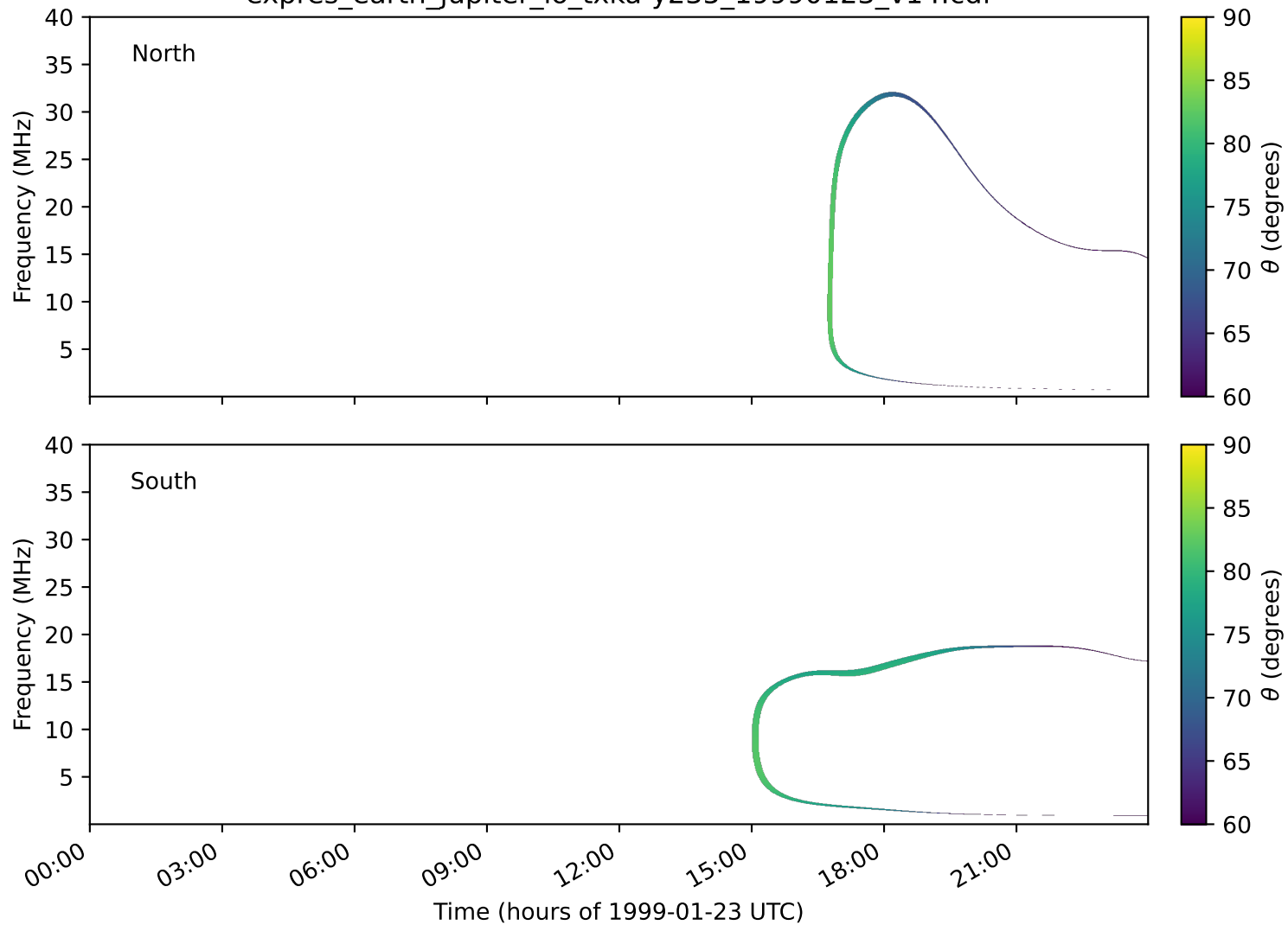
expres_earth_jupiter_io_txka-y235_19990123_v14.cdf
