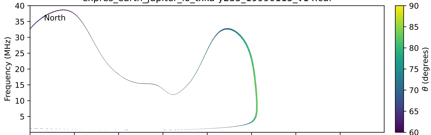
expres_earth_jupiter_io_txka-y235_19990115_v14.cdf
