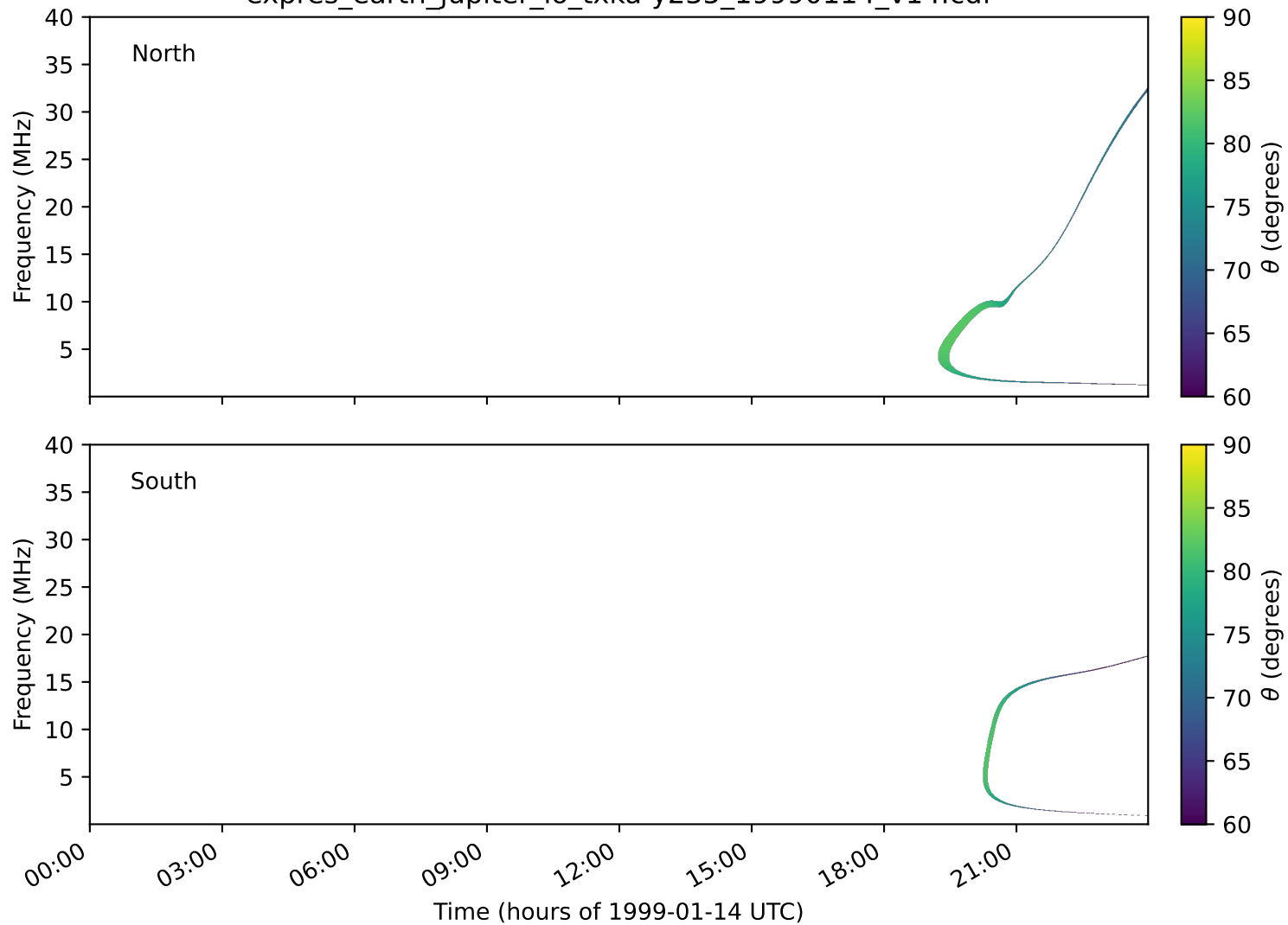
expres_earth_jupiter_io_txka-y235_19990114_v14.cdf
