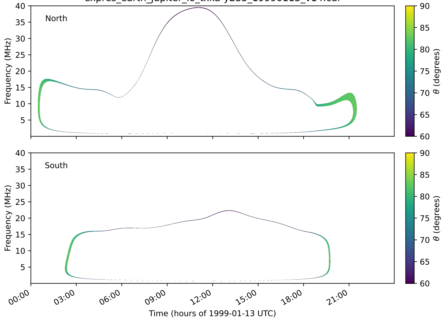
expres_earth_jupiter_io_txka-y235_19990113_v14.cdf
