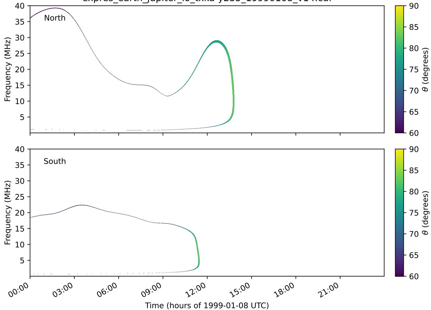
expres_earth_jupiter_io_txka-y235_19990108_v14.cdf
