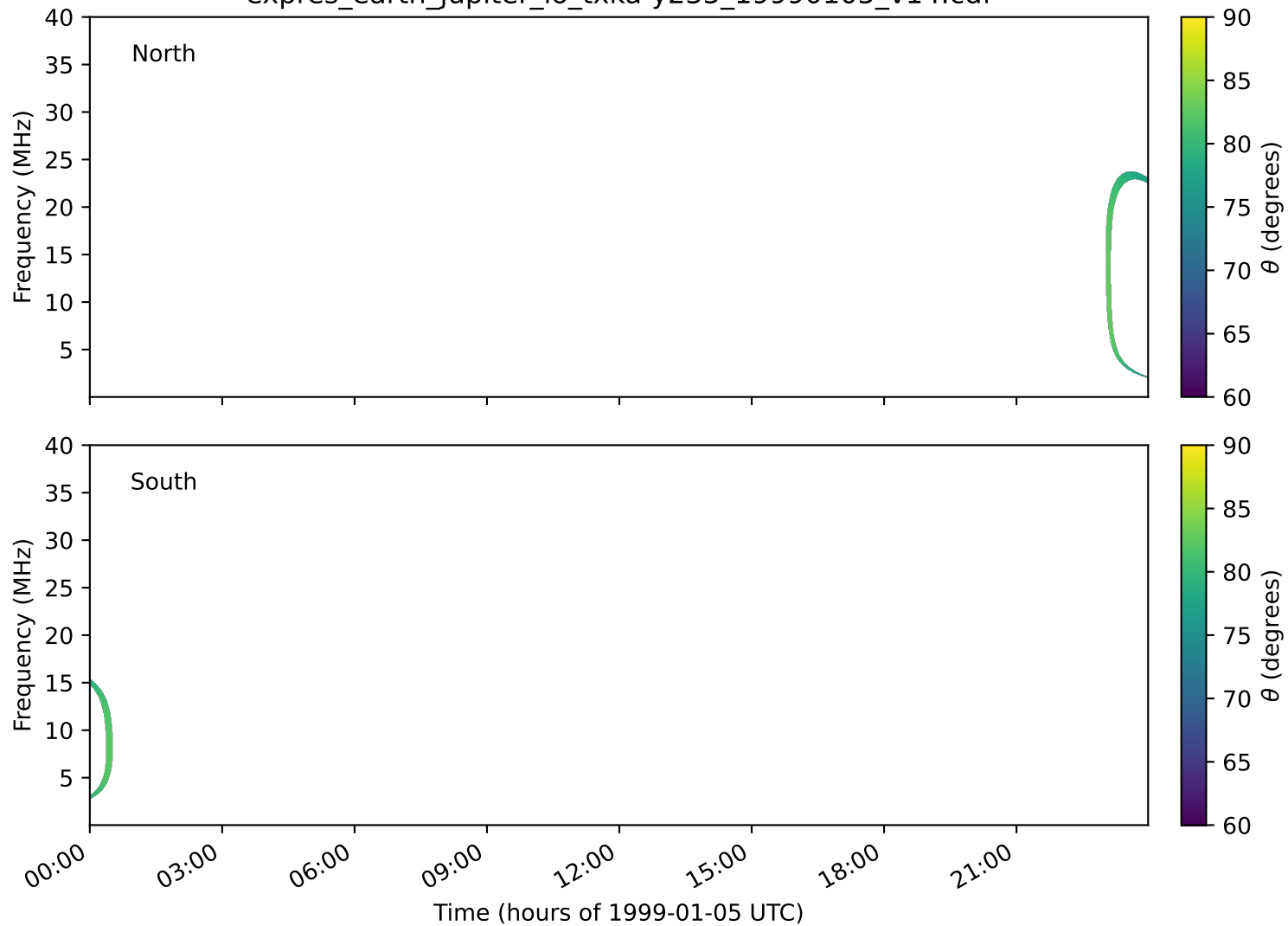
expres_earth_jupiter_io_txka-y235_19990105_v14.cdf
