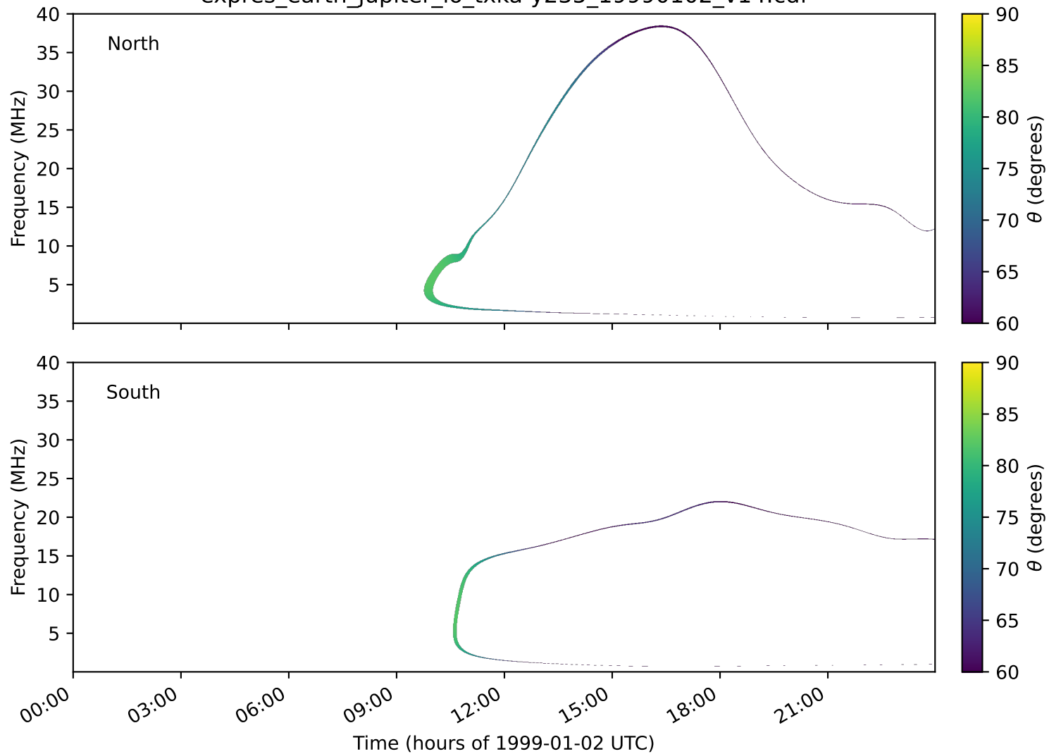
expres_earth_jupiter_io_txka-y235_19990102_v14.cdf
