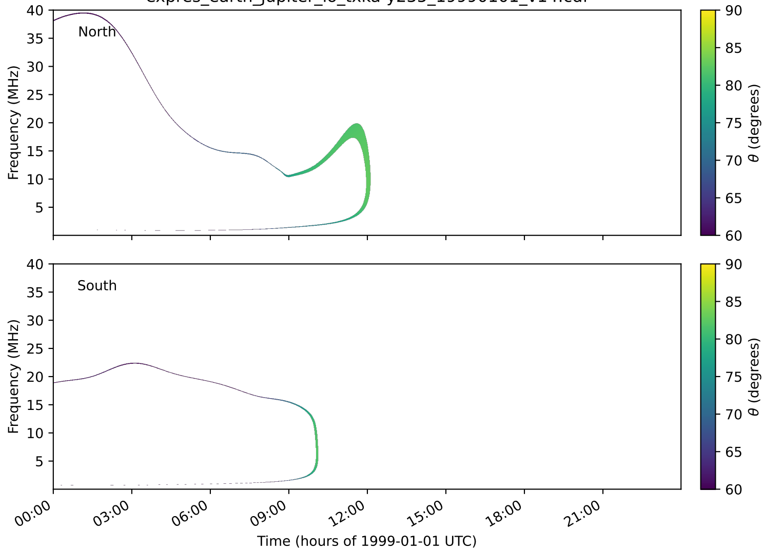
expres_earth_jupiter_io_txka-y235_19990101_v14.cdf
