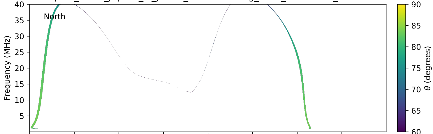
expres_earth_jupiter_io_jrm09_lossc-wid1deg_3kev_19990129_v11.cdf
