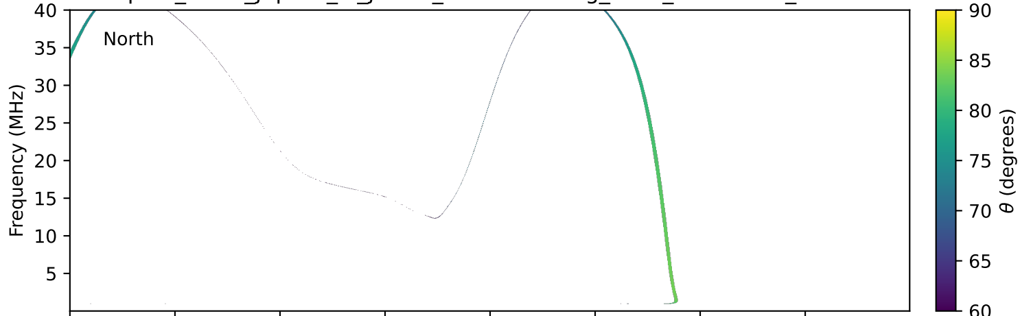
expres_earth_jupiter_io_jrm09_lossc-wid1deg_3kev_19990122_v11.cdf
