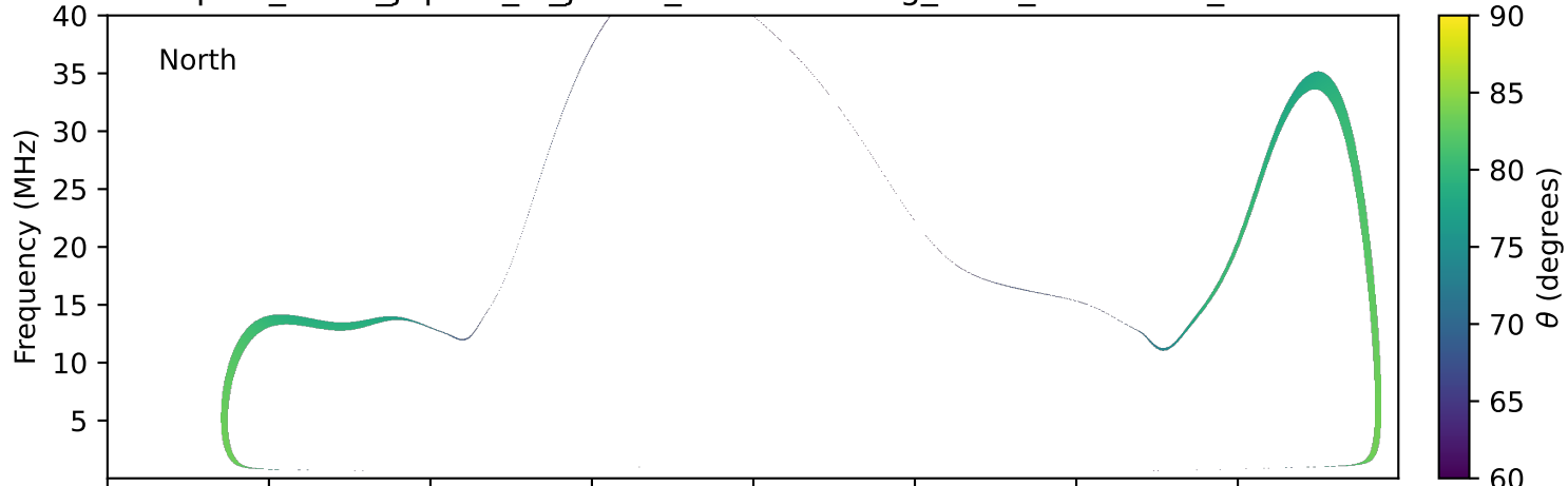
expres_earth_jupiter_io_jrm09_lossc-wid1deg_3kev_19990120_v11.cdf
