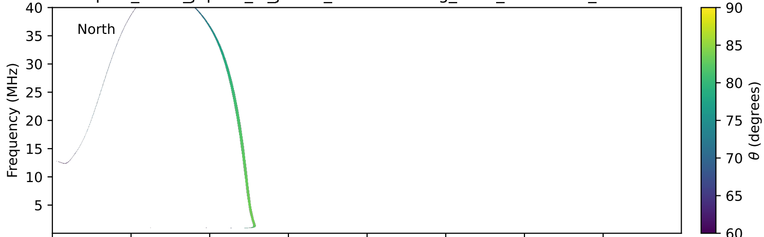
expres_earth_jupiter_io_jrm09_lossc-wid1deg_3kev_19990110_v11.cdf
