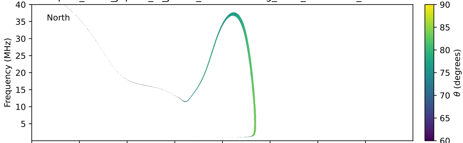
expres_earth_jupiter_io_jrm09_lossc-wid1deg_3kev_19990108_v11.cdf
