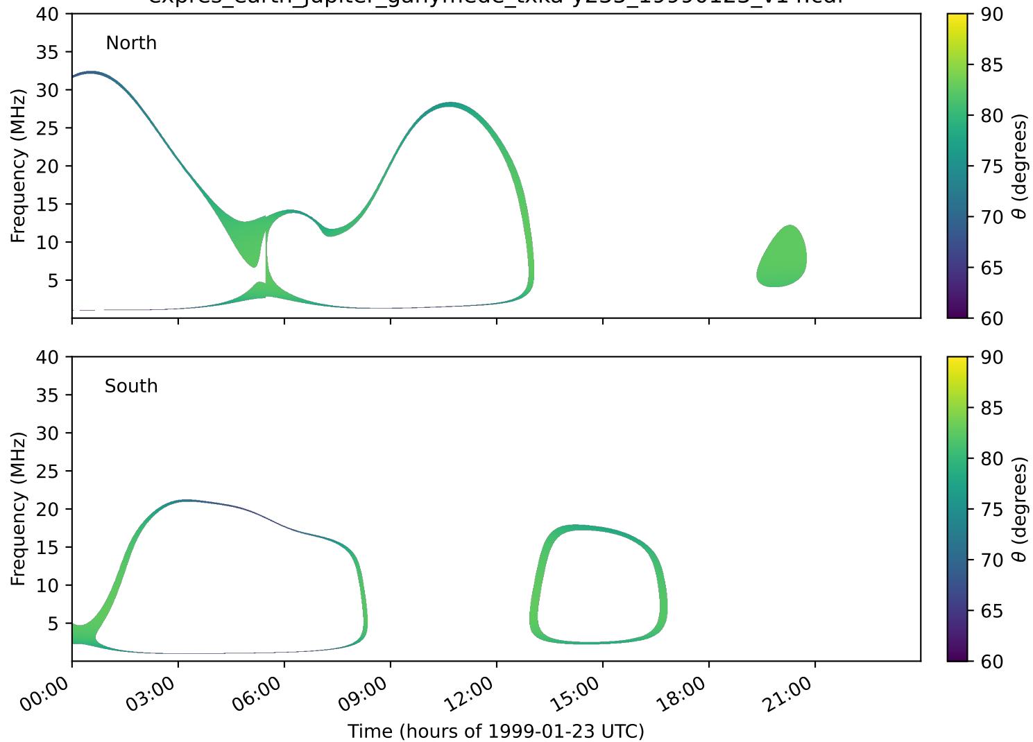
expres_earth_jupiter_ganymede_txka-y235_19990123_v14.cdf
