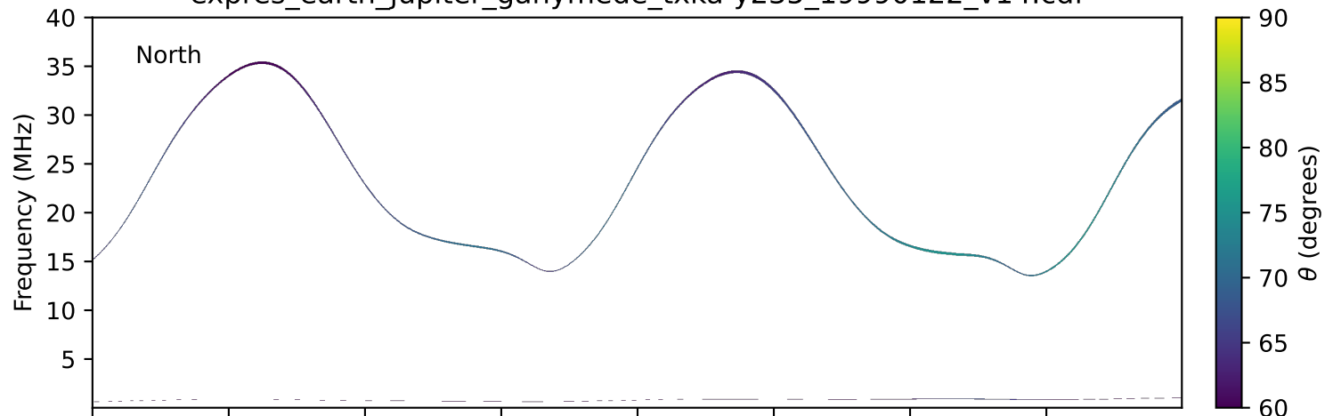
expres_earth_jupiter_ganymede_txka-y235_19990122_v14.cdf
