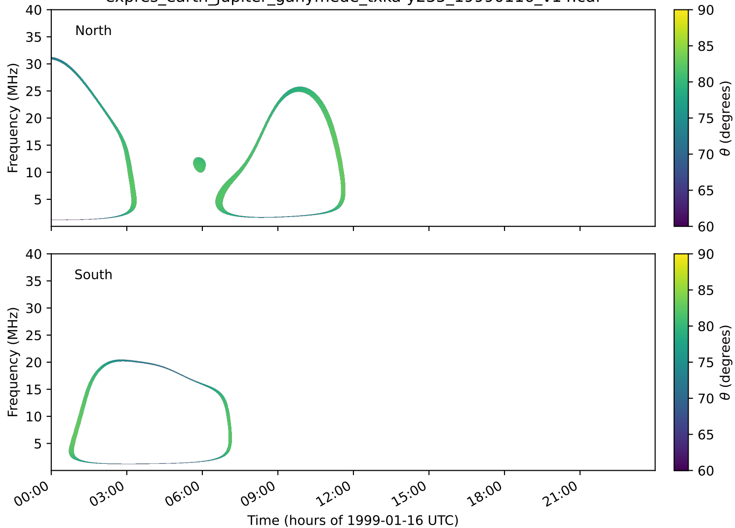
expres_earth_jupiter_ganymede_txka-y235_19990116_v14.cdf
