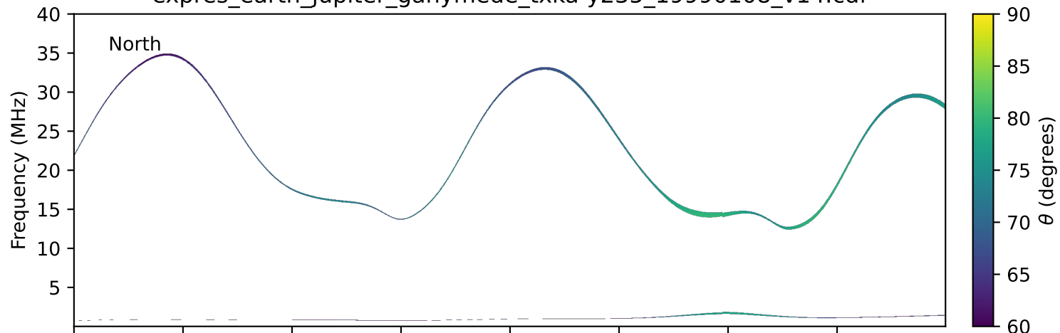
expres_earth_jupiter_ganymede_txka-y235_19990108_v14.cdf
