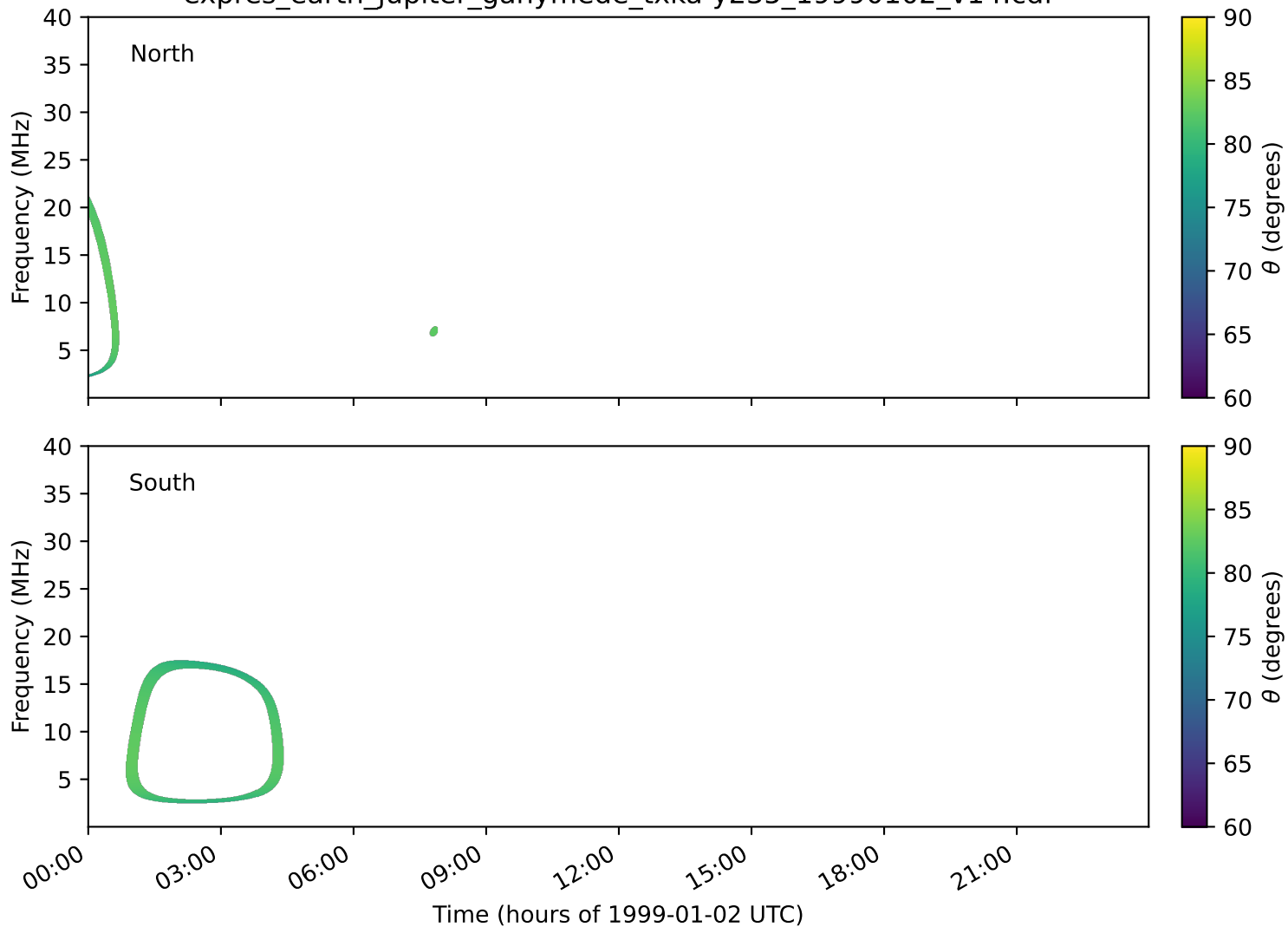
expres_earth_jupiter_ganymede_txka-y235_19990102_v14.cdf
