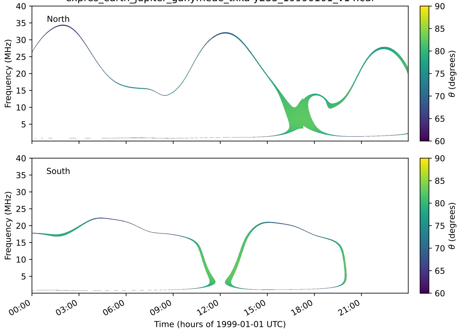
expres_earth_jupiter_ganymede_txka-y235_19990101_v14.cdf
