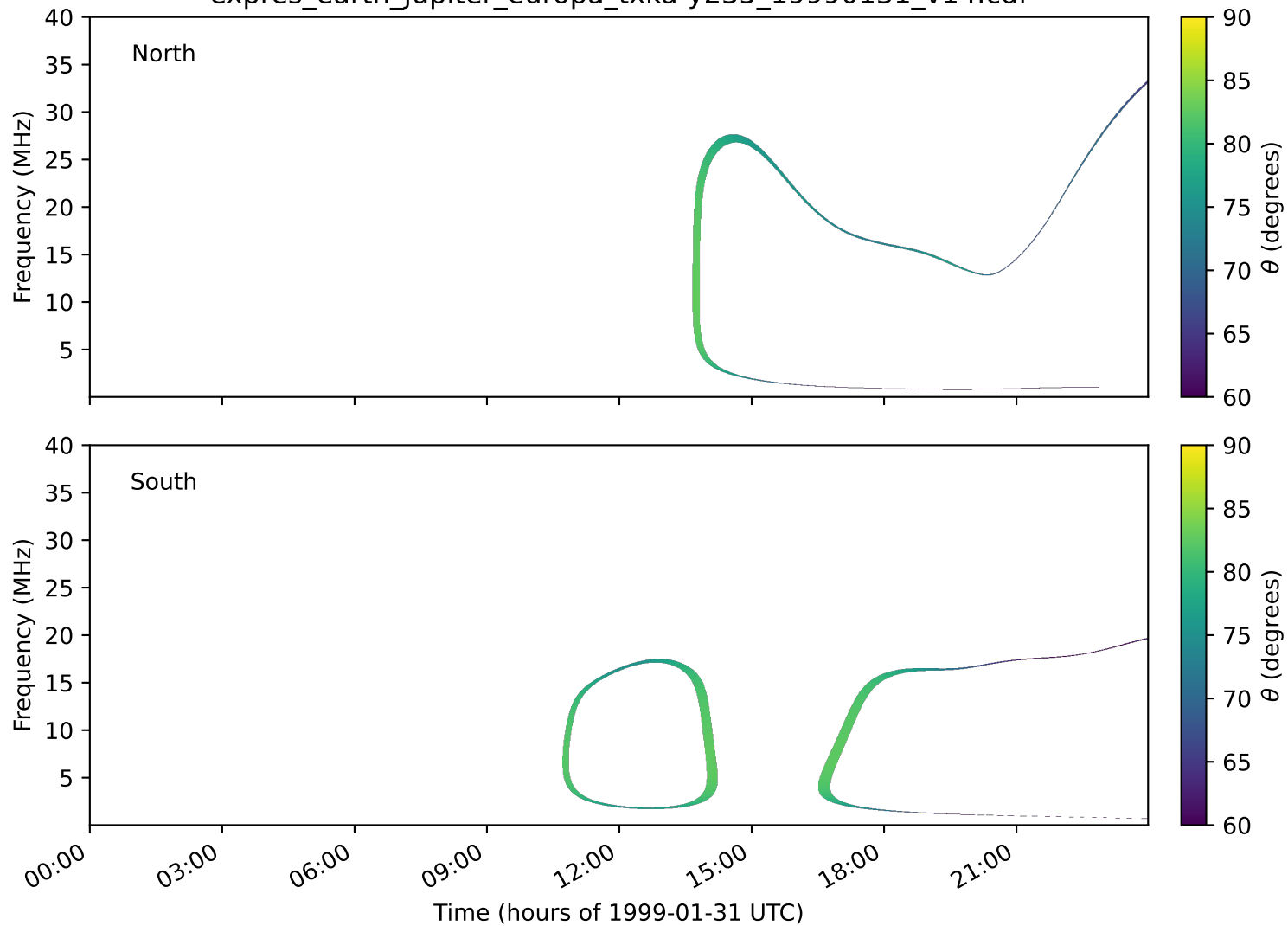
expres_earth_jupiter_europa_txka-y235_19990131_v14.cdf
