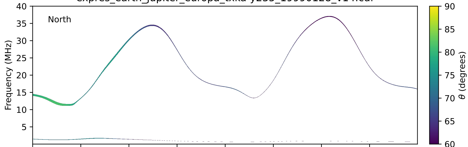
expres_earth_jupiter_europa_txka-y235_19990128_v14.cdf
