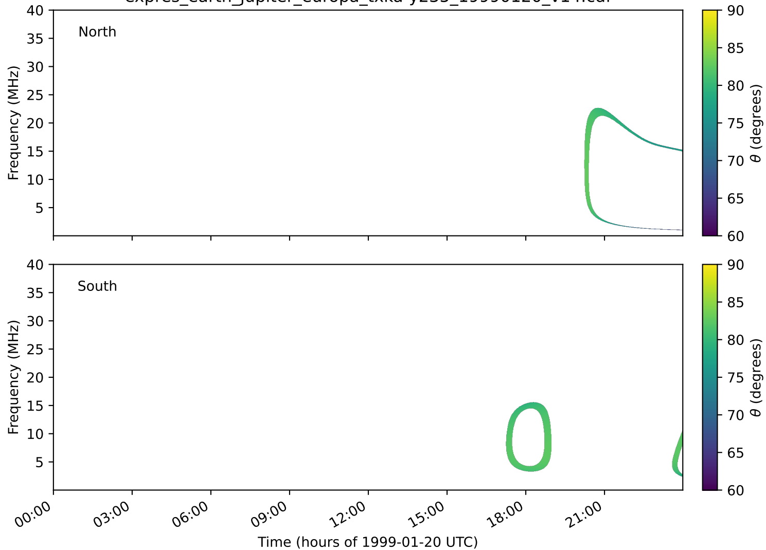
expres_earth_jupiter_europa_txka-y235_19990120_v14.cdf
