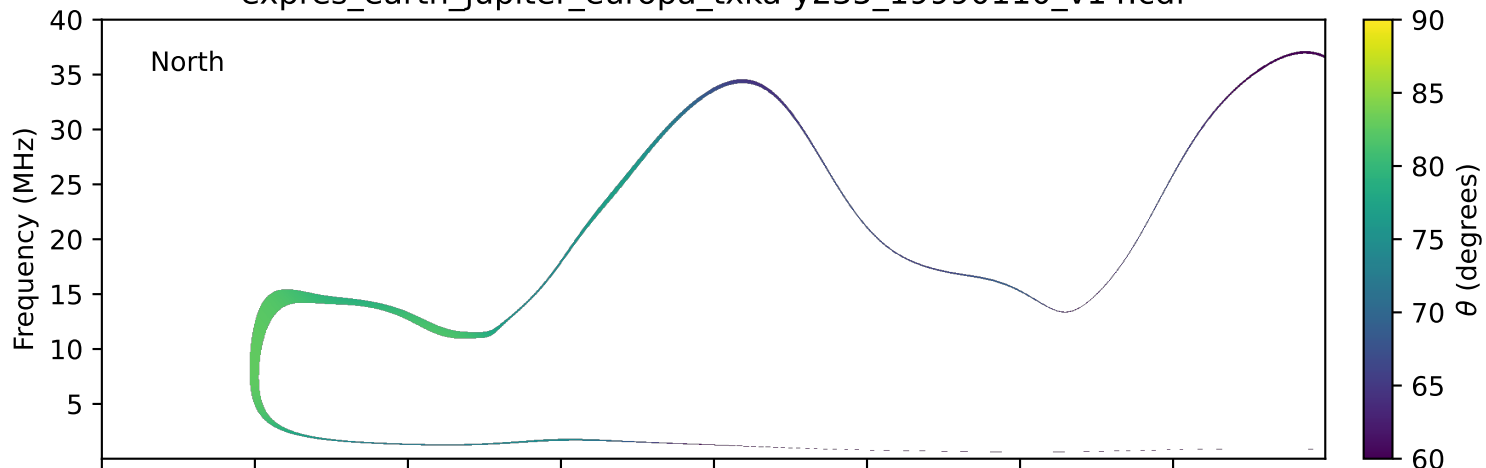
expres_earth_jupiter_europa_txka-y235_19990110_v14.cdf
