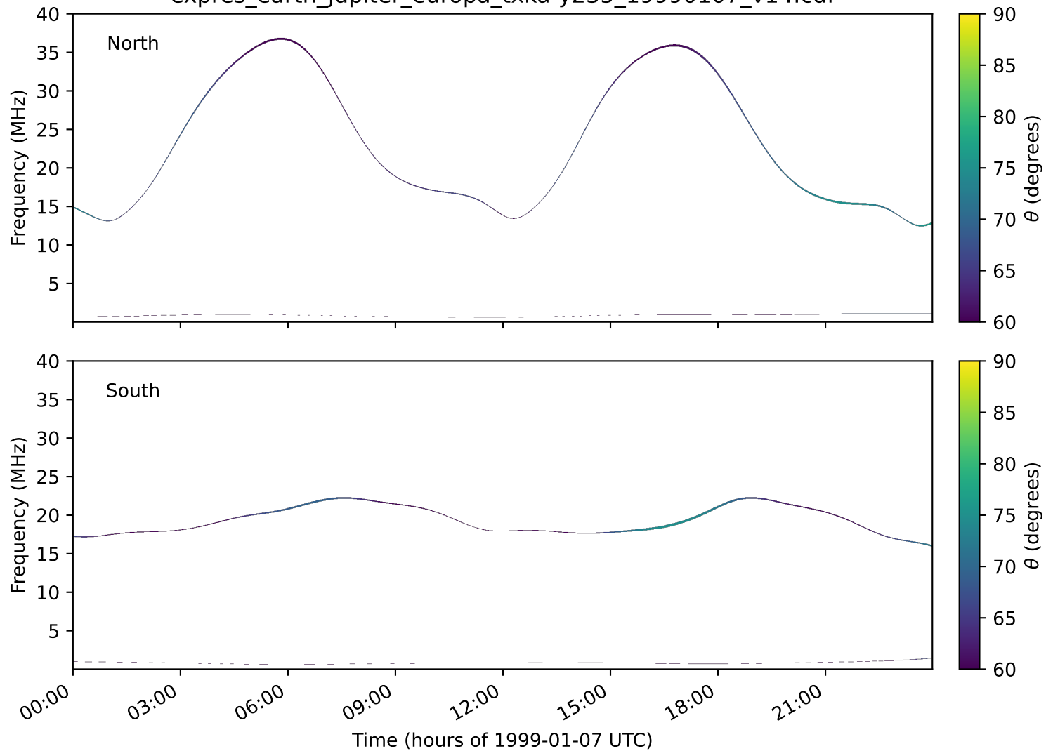
expres_earth_jupiter_europa_txka-y235_19990107_v14.cdf
