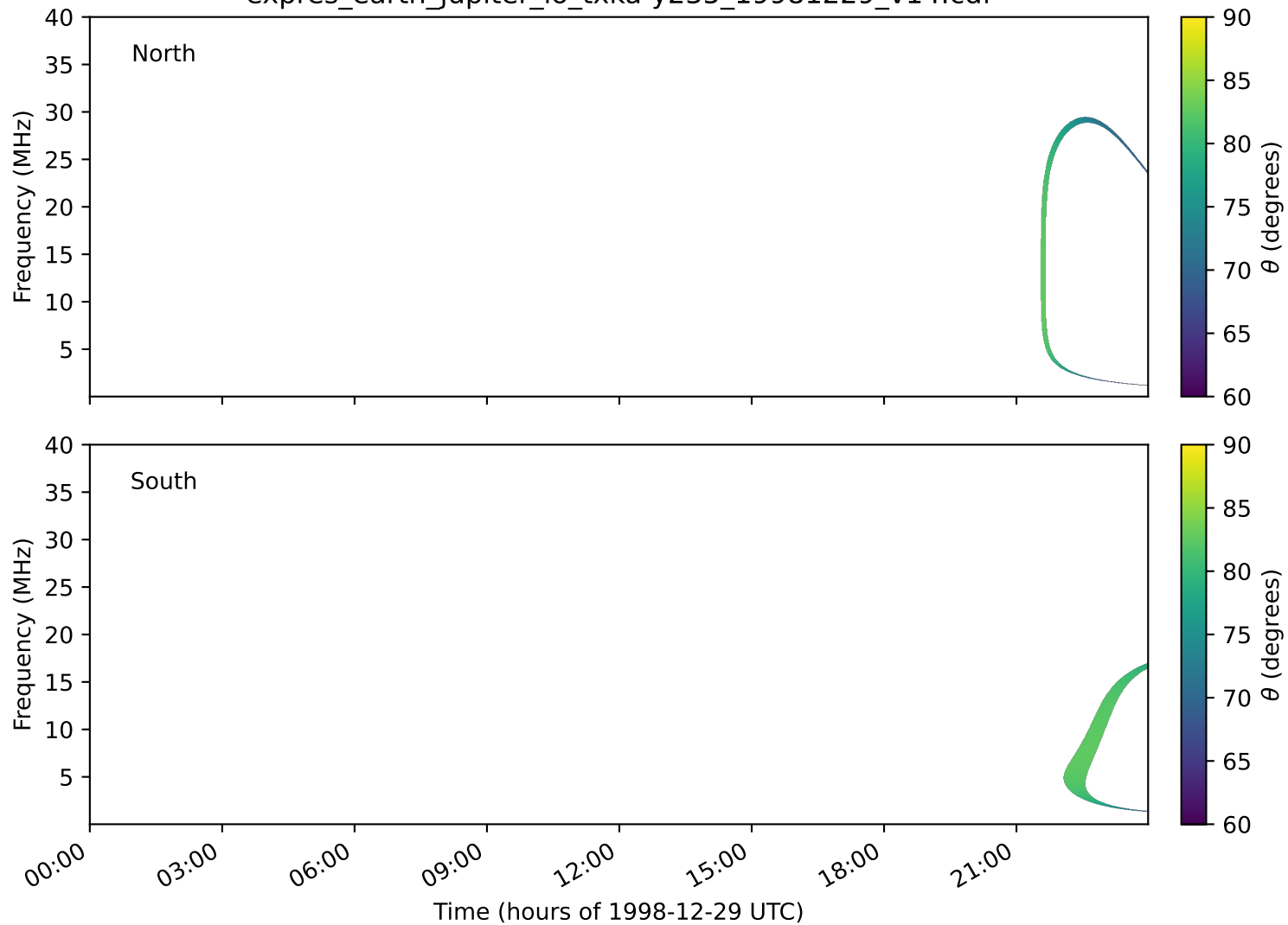
expres_earth_jupiter_io_txka-y235_19981229_v14.cdf
