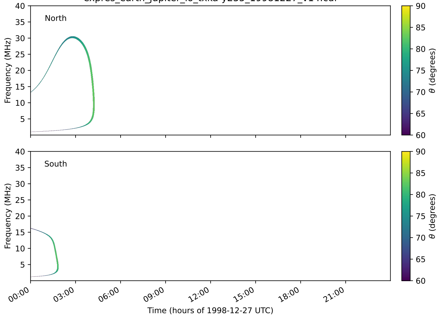
expres_earth_jupiter_io_txka-y235_19981227_v14.cdf
