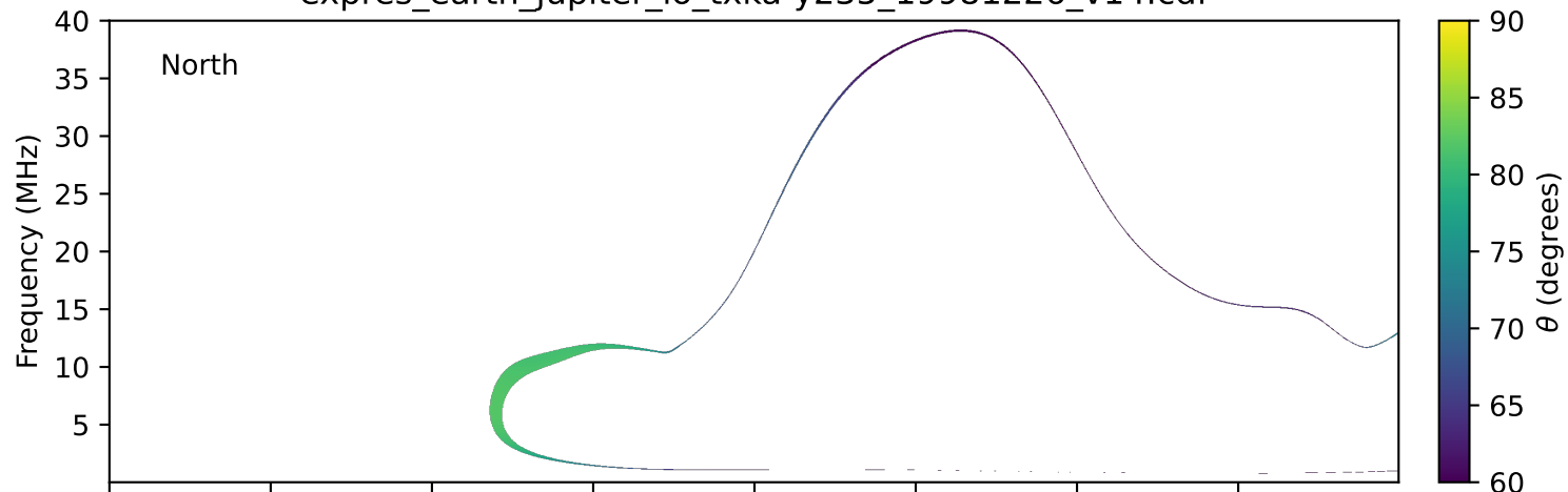
expres_earth_jupiter_io_txka-y235_19981226_v14.cdf
