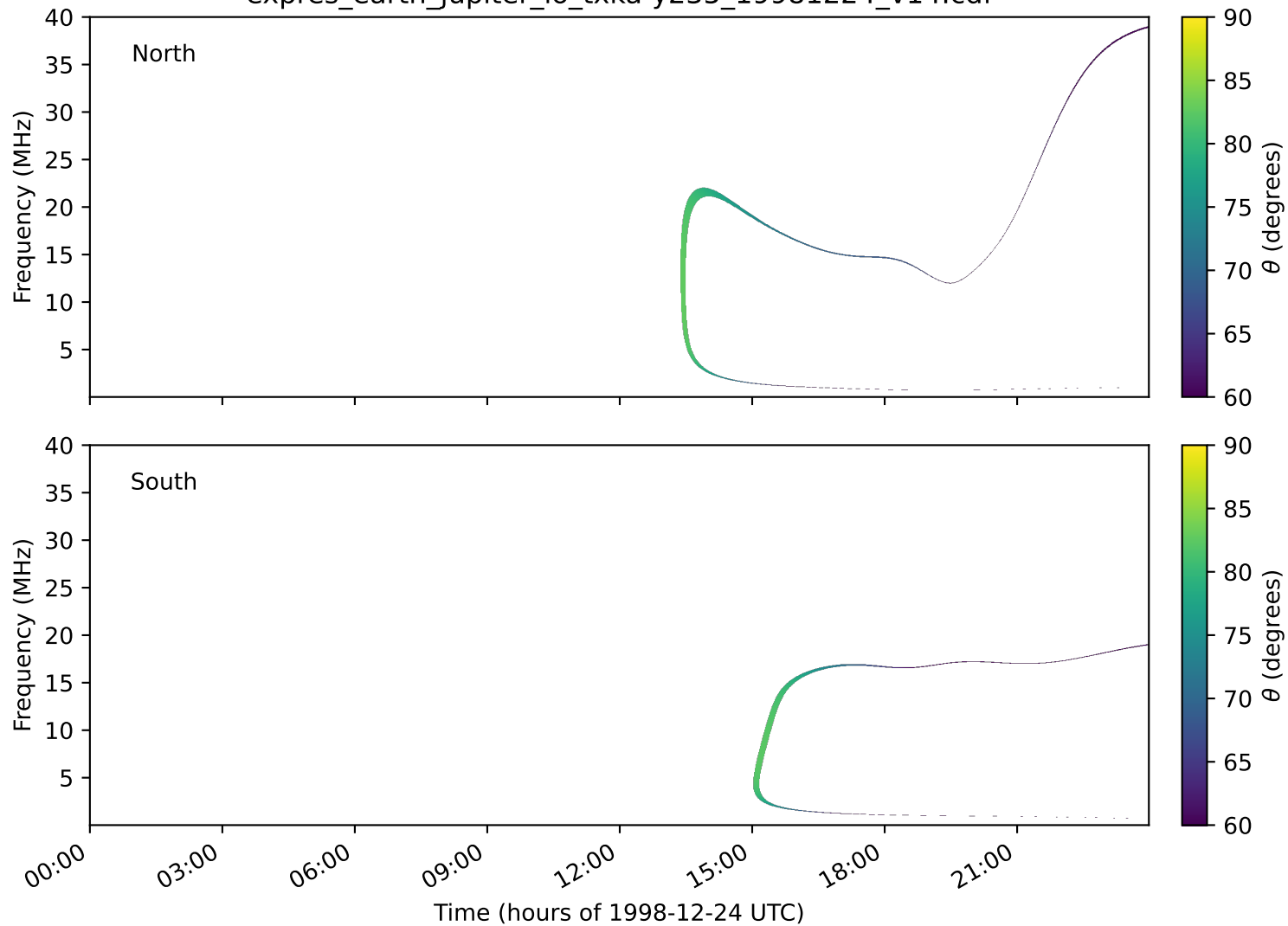
expres_earth_jupiter_io_txka-y235_19981224_v14.cdf
