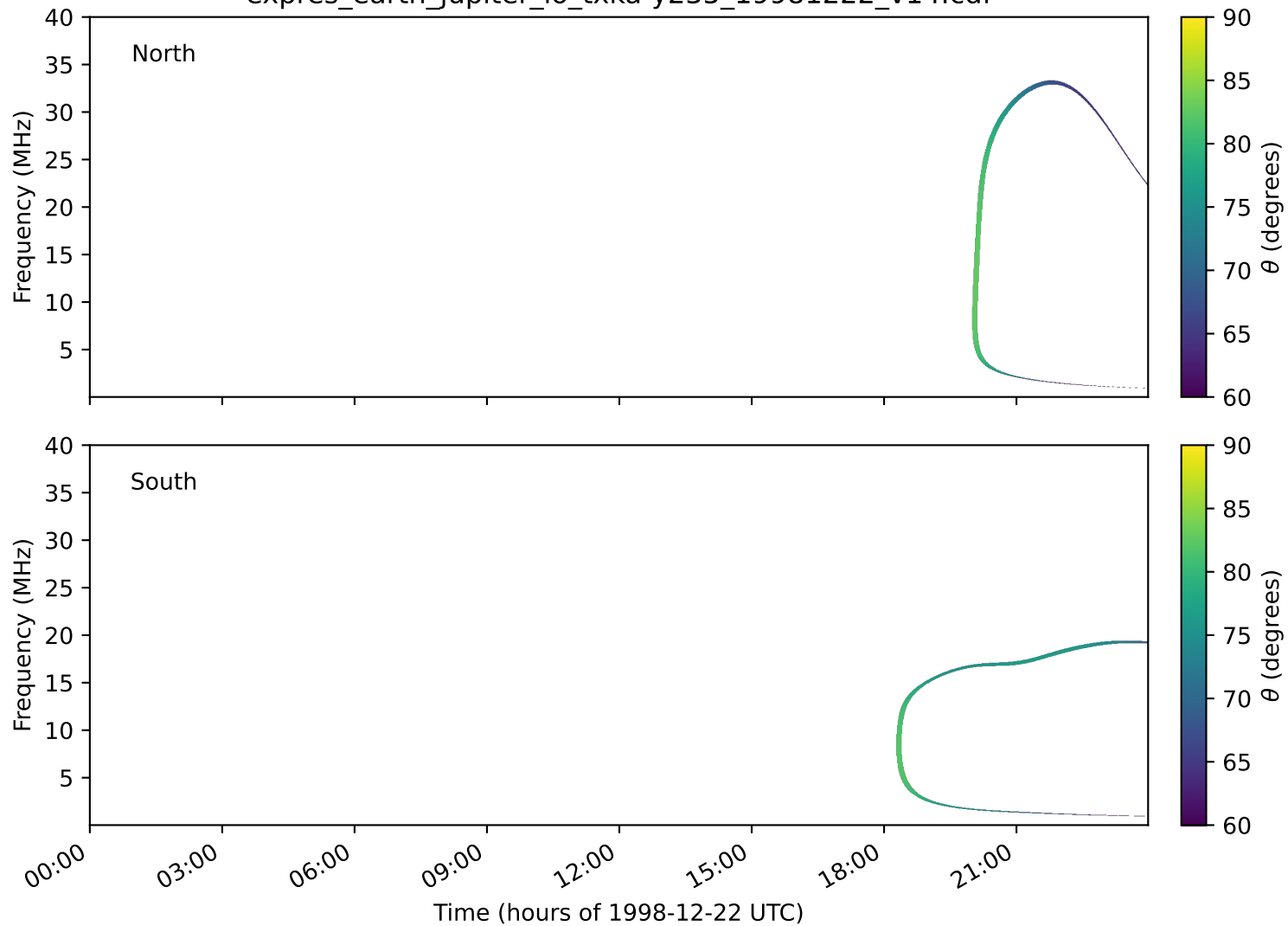
expres_earth_jupiter_io_txka-y235_19981222_v14.cdf
