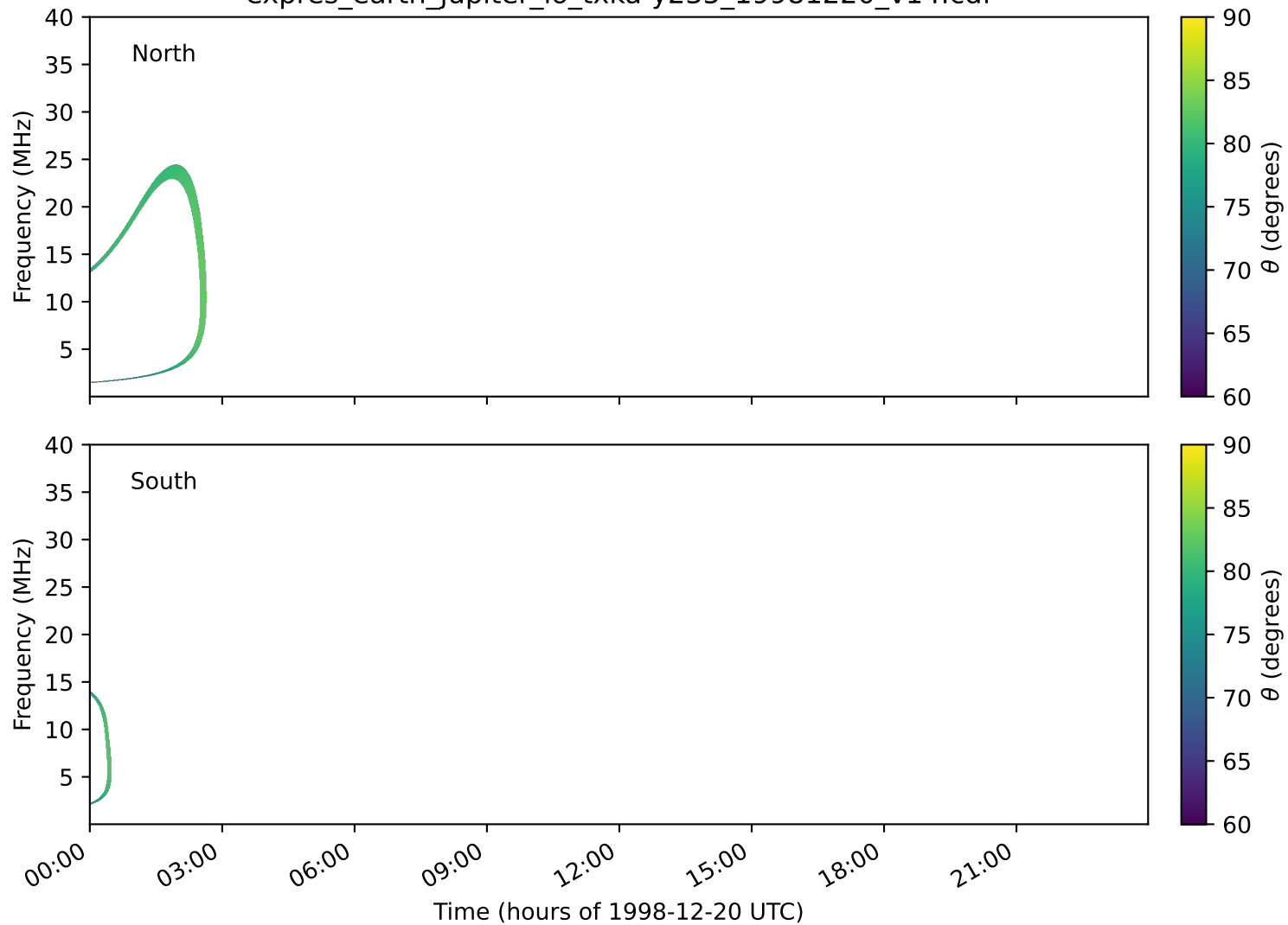
expres_earth_jupiter_io_txka-y235_19981220_v14.cdf
