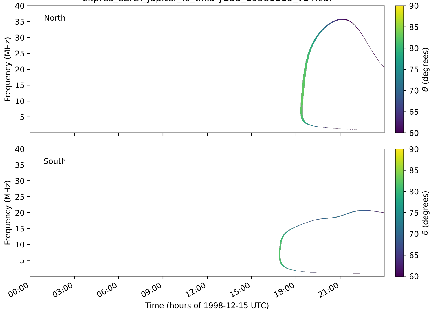
expres_earth_jupiter_io_txka-y235_19981215_v14.cdf
