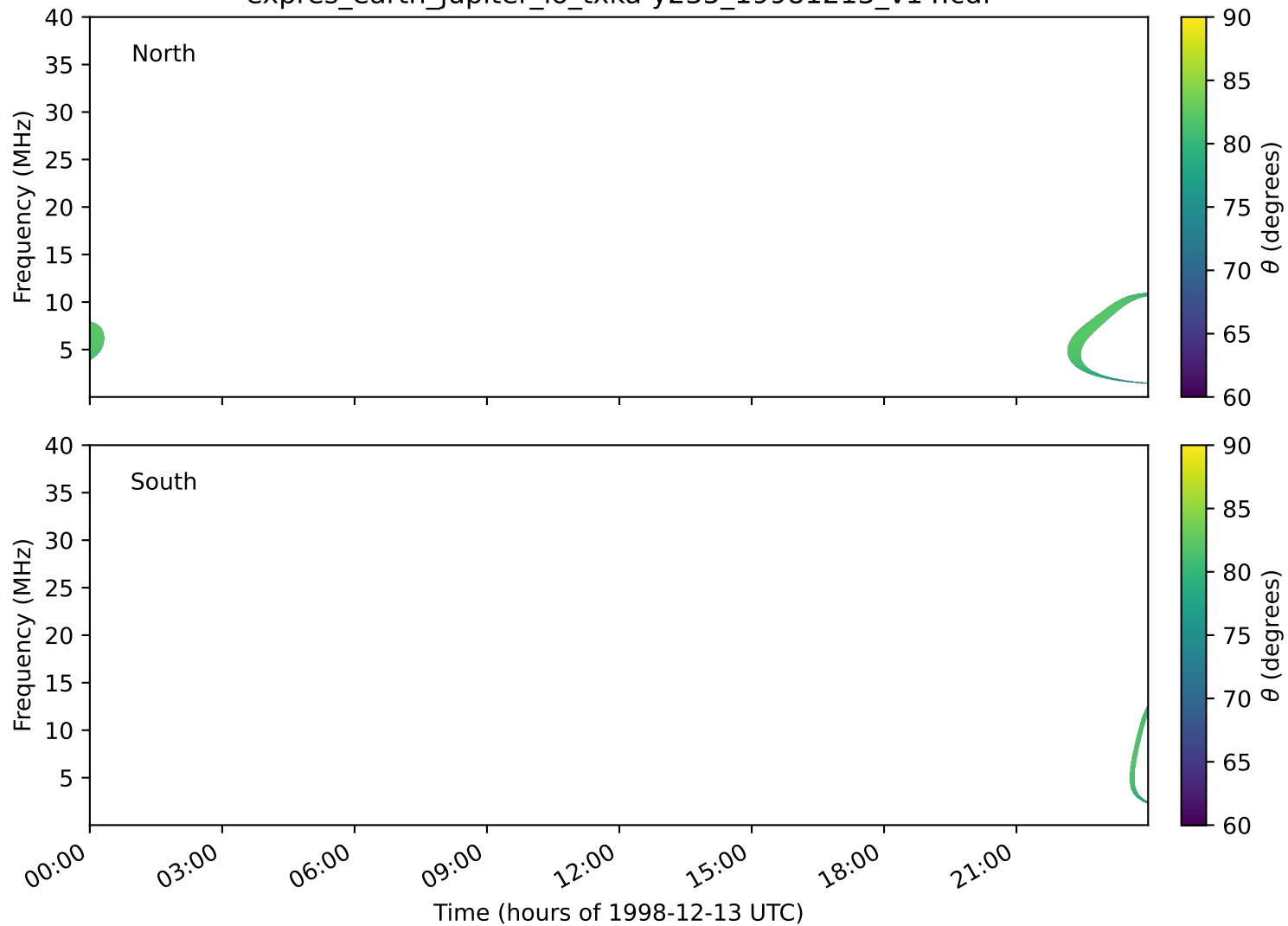
expres_earth_jupiter_io_txka-y235_19981213_v14.cdf
