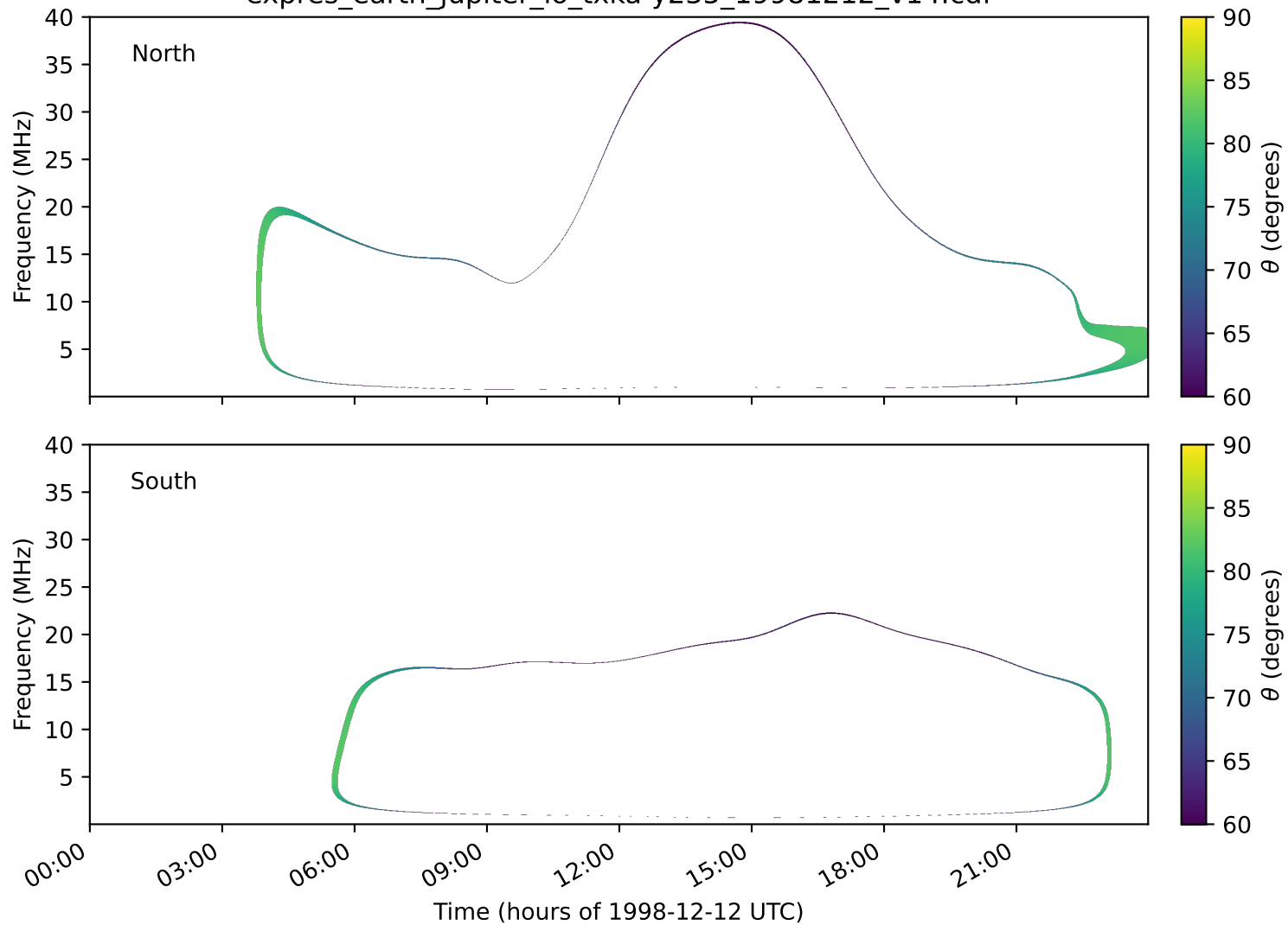
expres_earth_jupiter_io_txka-y235_19981212_v14.cdf
