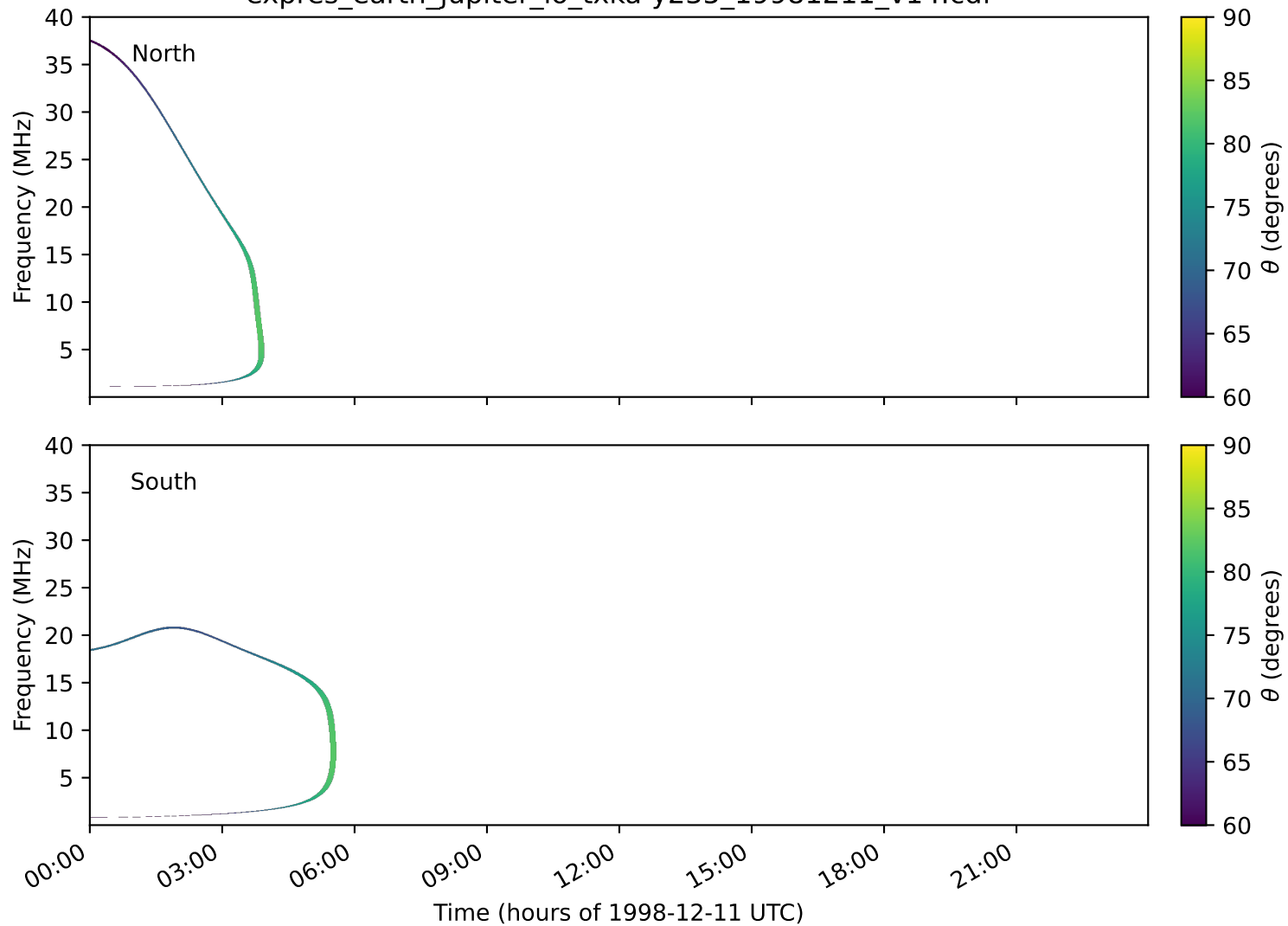
expres_earth_jupiter_io_txka-y235_19981211_v14.cdf
