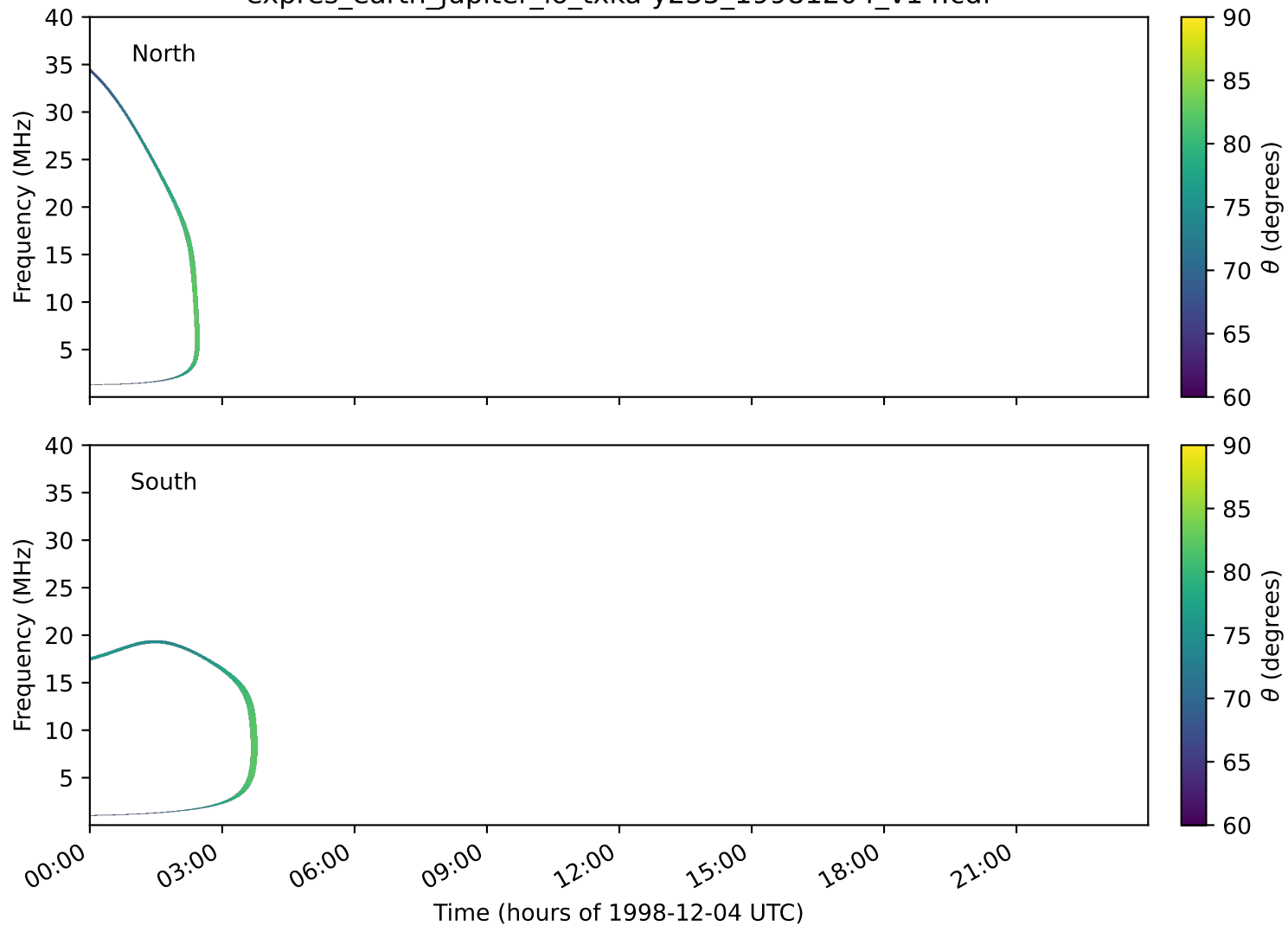
expres_earth_jupiter_io_txka-y235_19981204_v14.cdf
