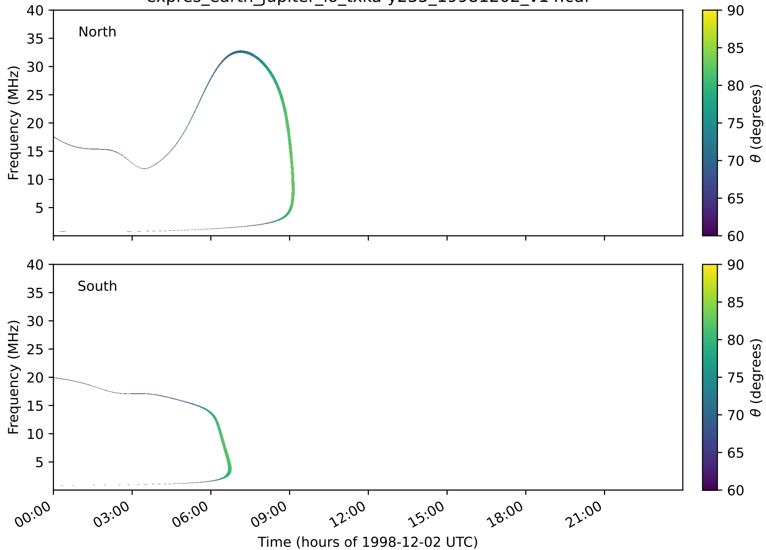
expres_earth_jupiter_io_txka-y235_19981202_v14.cdf
