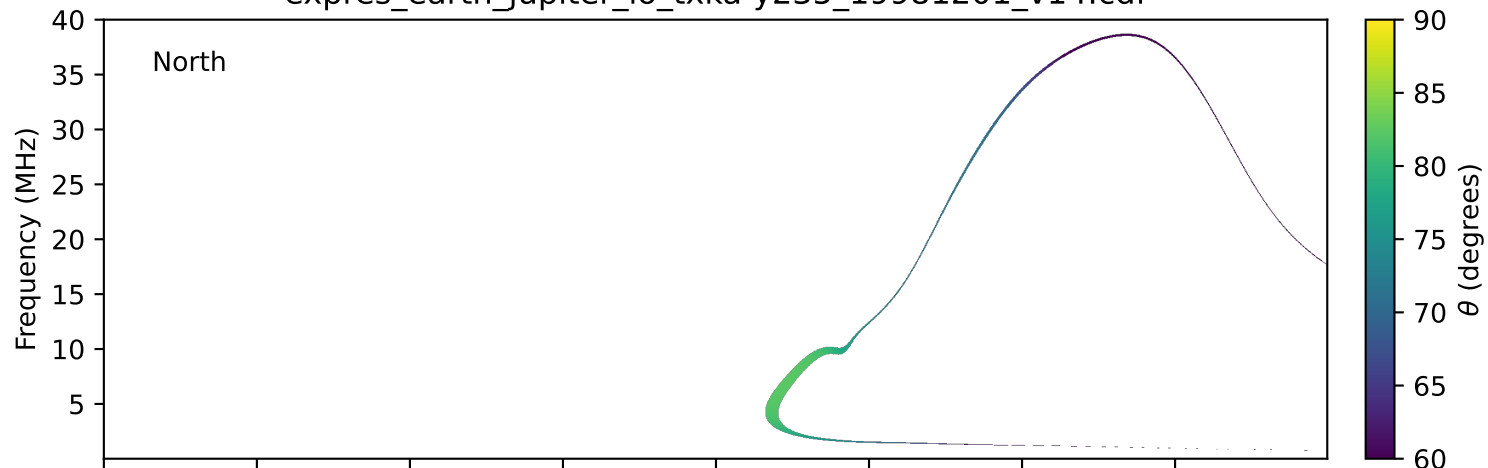
expres_earth_jupiter_io_txka-y235_19981201_v14.cdf
