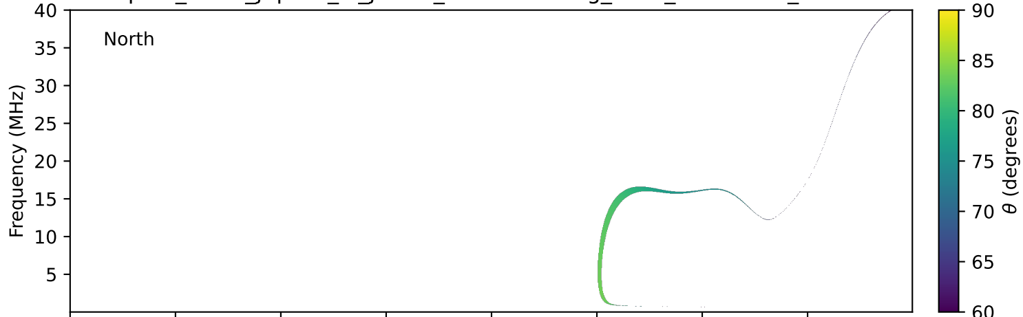
expres_earth_jupiter_io_jrm33_lossc-wid1deg_3kev_19981231_v11.cdf
