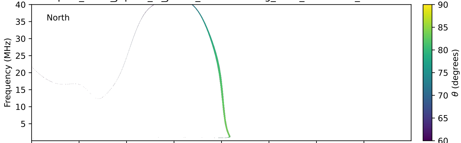
expres_earth_jupiter_io_jrm33_lossc-wid1deg_3kev_19981216_v11.cdf
